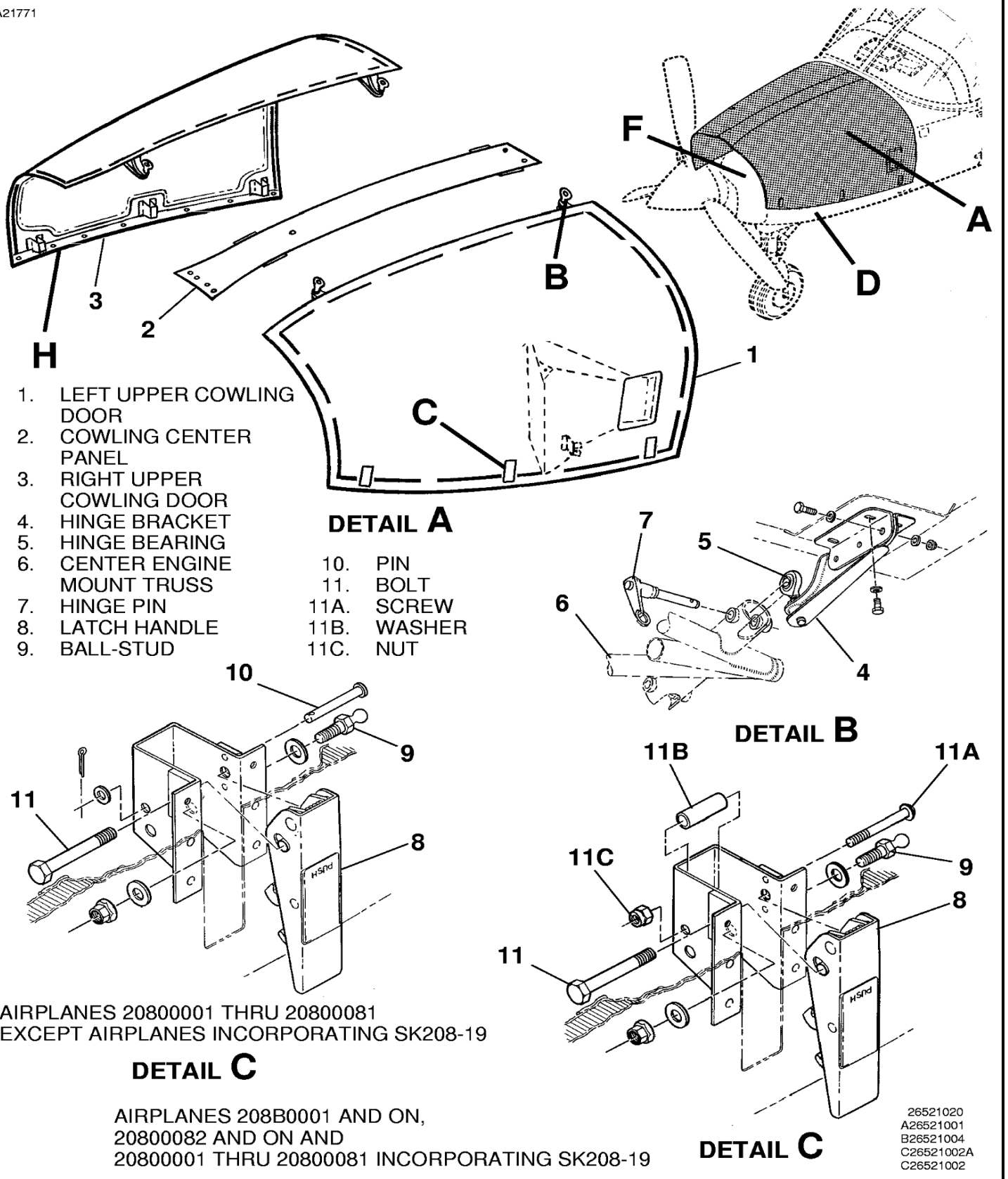
Figure 201 : Sheet 1 : Cowling and Nose Cap Installation
