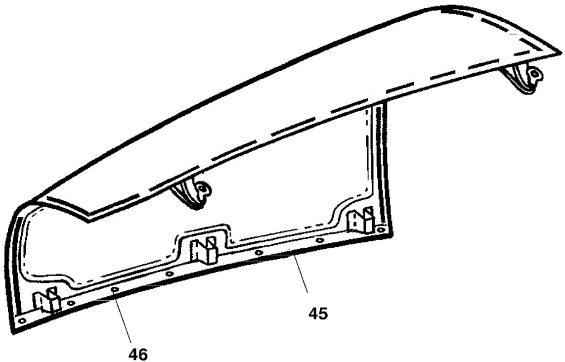
DETAIL H TYPICAL RUB STRIP INSTALLATION
