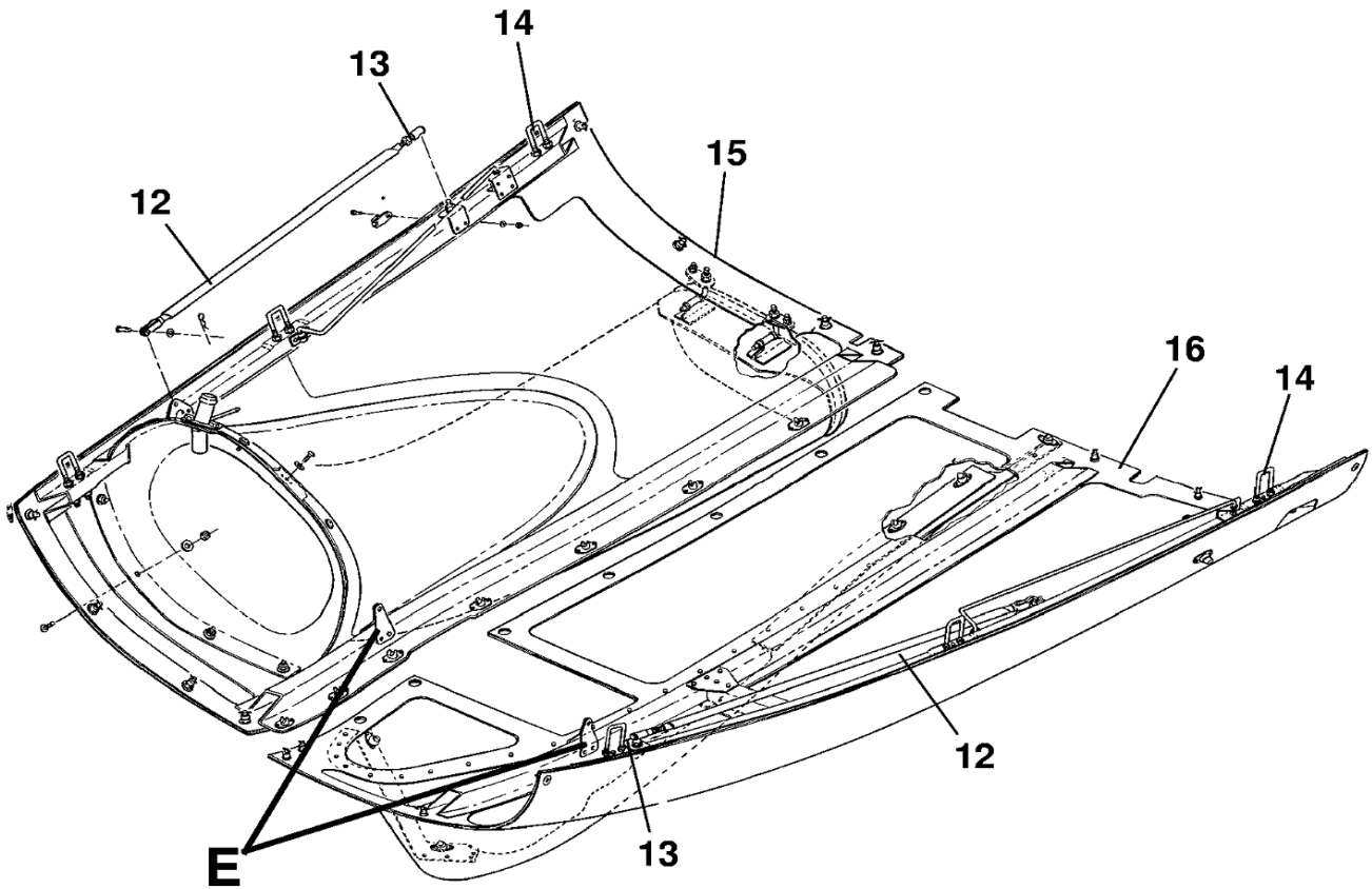
DETAIL D
