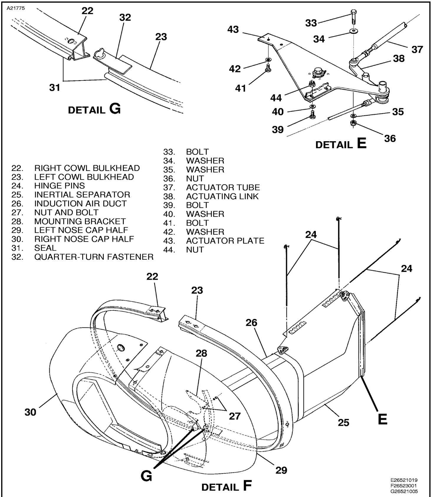
Figure 201 : Sheet 3 : Cowling and Nose Cap Installation
